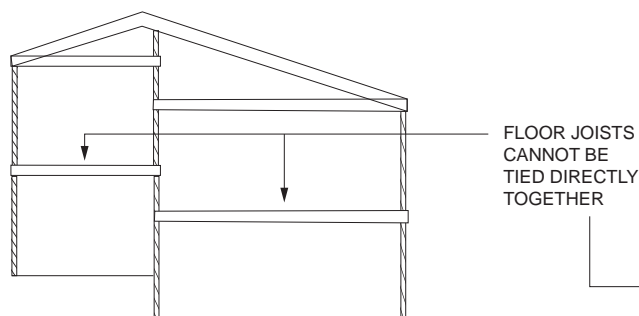
SECTION VIEW
